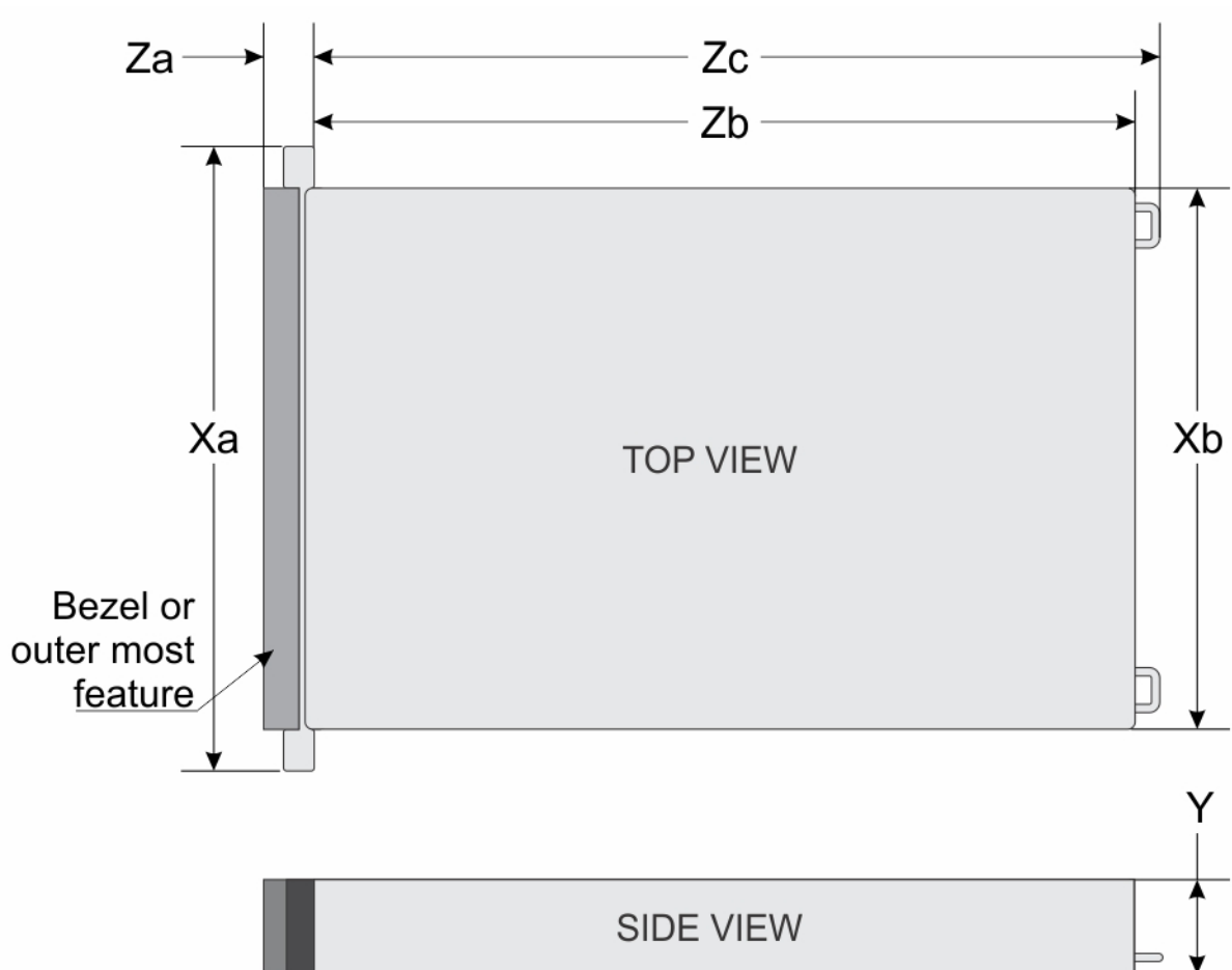
Figure 51. Chassis dimensions
