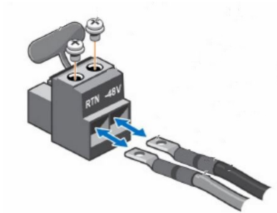
Figure 35. DC PSU power cord*
