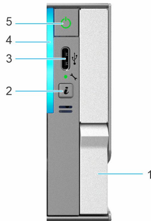
Figure 15. Right Control Panel (RCP) - Primary of R7715
