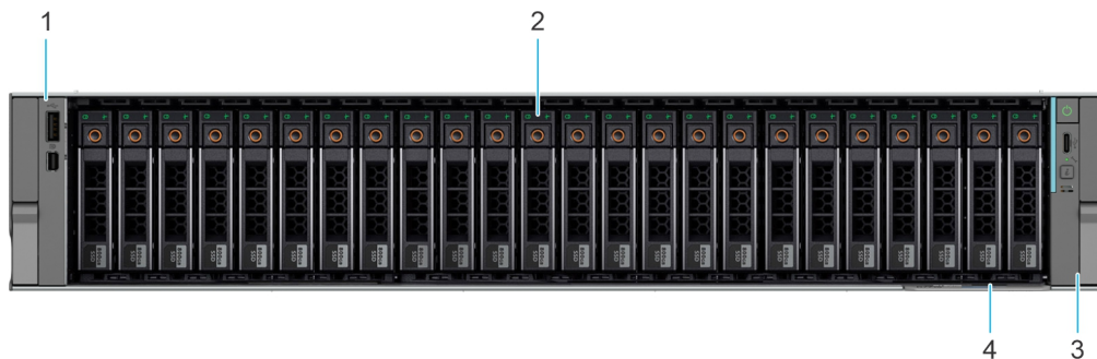
Figure 9. Front view of 24 x 2.5-inch SAS/SATA drives system
