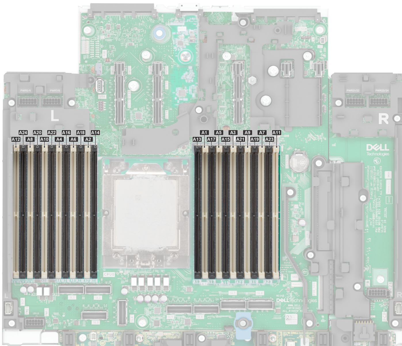
Figure 22. Memory channels
