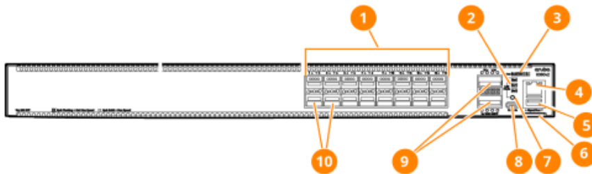
Figure 7 Chassis and Port LEDs for the Aruba 8360-16Y2C (JL702C/JL703C/JL718C)
