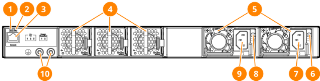
Figure 1 Back of HPE Aruba Networking 8360 Rev A & C Switches except 8360-48Y6C
