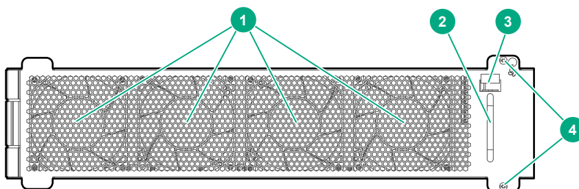
Figure 14: Fan tray
