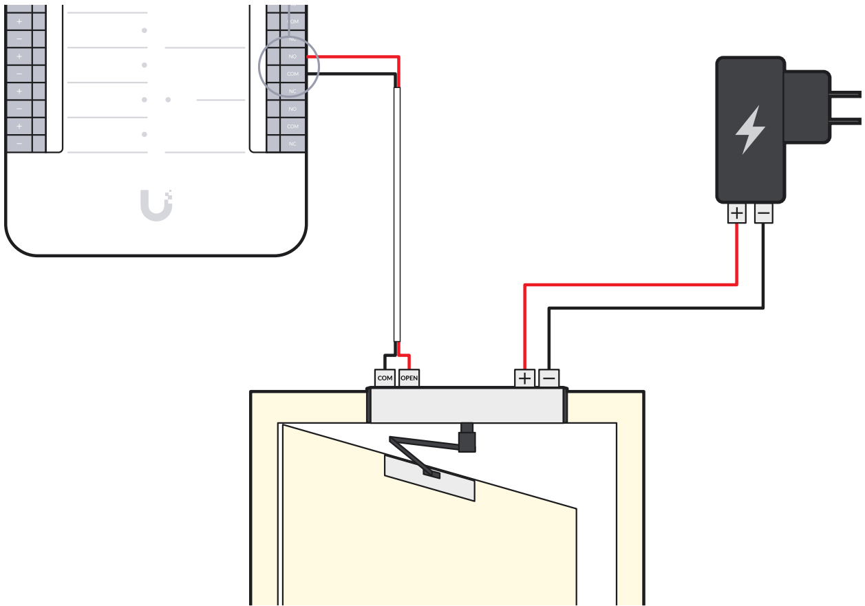
Door Operator
