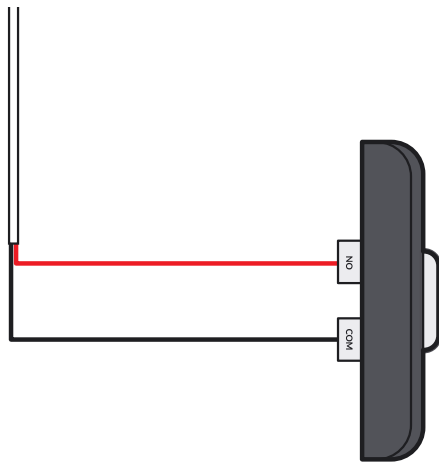
Push Button
