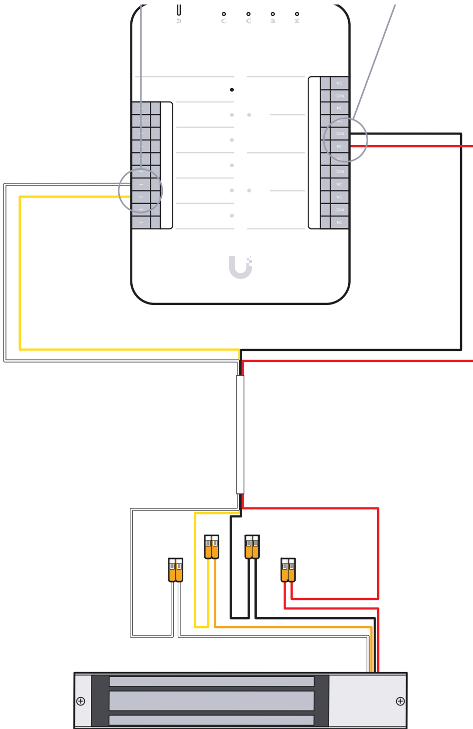
Access Lock Magnetic (Fail-Safe Lock)
