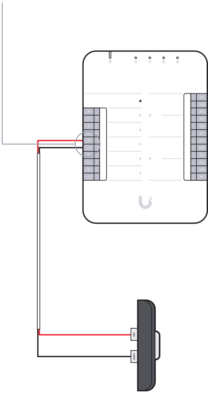
Push Button
