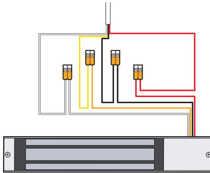
Access Lock Magnetic (Fail-Safe Lock)
