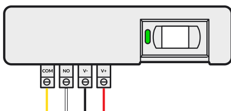
Motion Sensor
