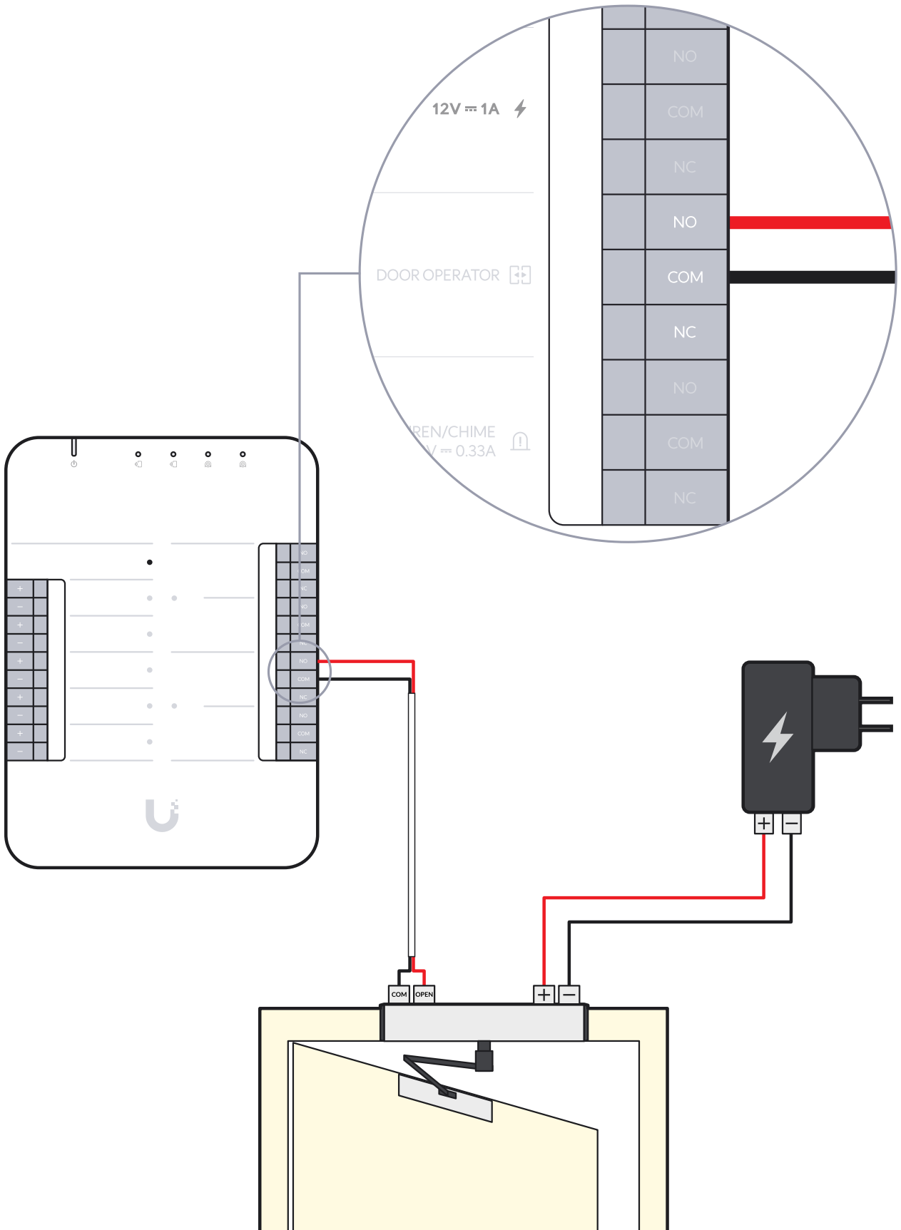
Door Operator
