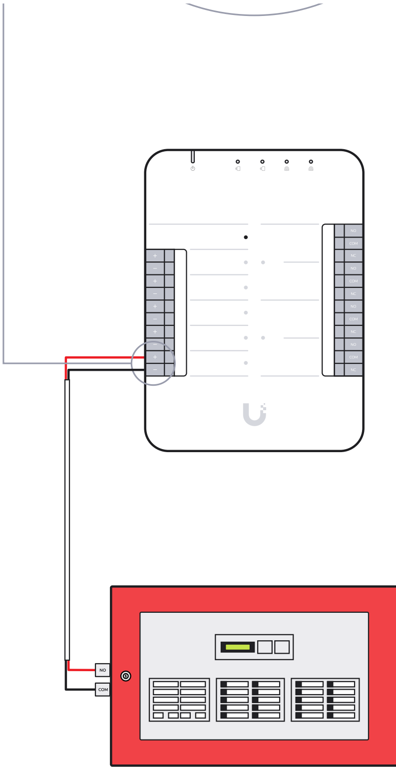
Fire Panel
