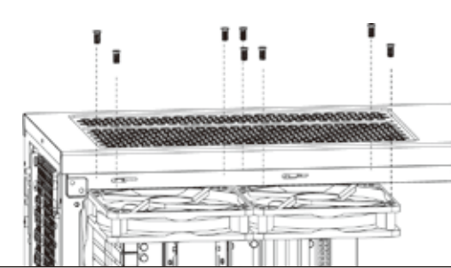
(7c) Top Case Fans
